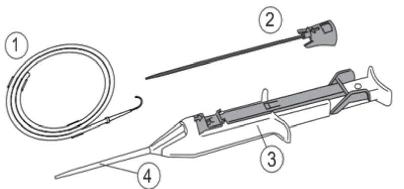
Figure 2.1 FemoSeal™ VCS Unit with the Guidewire and Dilator
